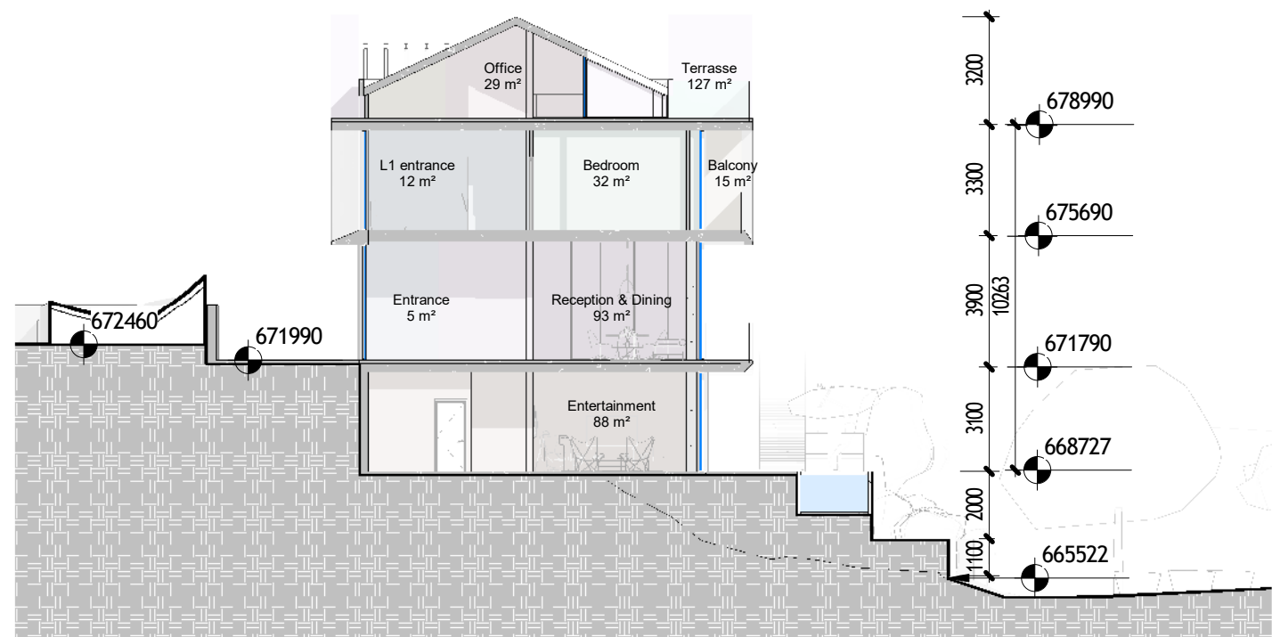
Section 1
