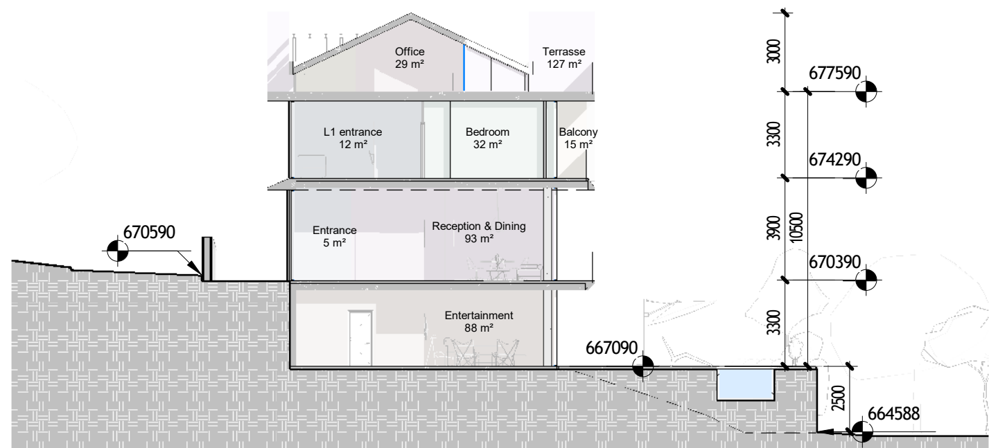
Section 2
