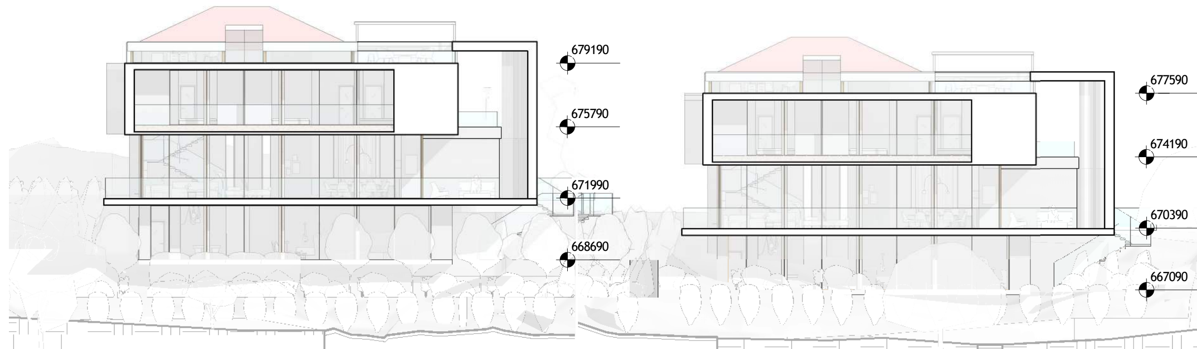
South Elevation
